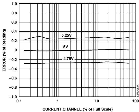
Figure 10. PSR with Internal Reference, PF = 1
