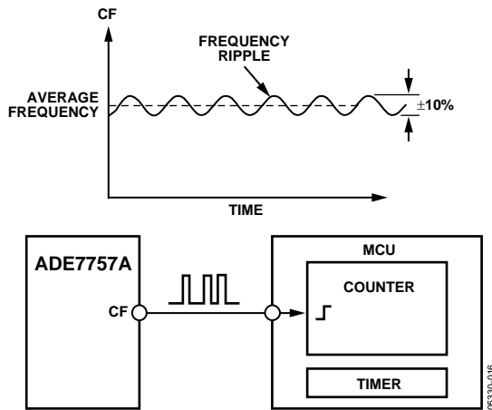
Figure 26. Interfacing the ADE7757A to an MCU
